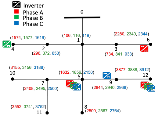
Fig. 6. Multiphase IEEE 13-bus distribution feeder.
