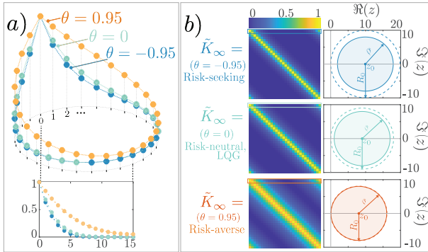
Fig. 1: Steady-state normalized optimal LEQG control gain \tilde{K}_\infty := K_\infty/K_\infty(0,0) for the case study in Section V-B with n = 30 . \tilde{K}_\infty is plotted for different \theta , as indicated. a) \tilde{k} as a function in the discrete circle \mathbb{Z}_{30} . The change in the spatial decay rate of the gain at different values of \theta is apparent in the lower panel. b) \tilde{K}_\infty : entries colored according to their respective values, following the colorbar. The second column shows the closed disk \mathcal{D} containing the spectrum \sigma_{\mathcal{R}}(\theta) and the largest concentric open disk where f(\cdot) := \sqrt{\cdot} is analytic in the complex plane.
