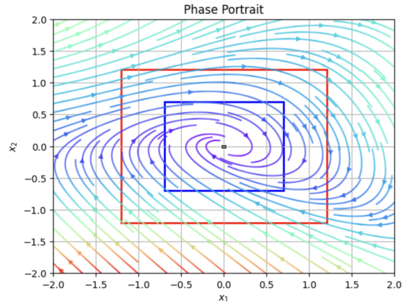
Fig. 3: Phase portrait of system (24), wherein the black box surrounds the region which we do not verify ( B_\varepsilon(x^*) ), the blue box represents surrounds the region which we verify in Algorithm 3 ( B_R(x^*) ), and the red box surrounds the region which trajectories that begin in the blue box do not leave ( B_{R'}(x^*) ).
