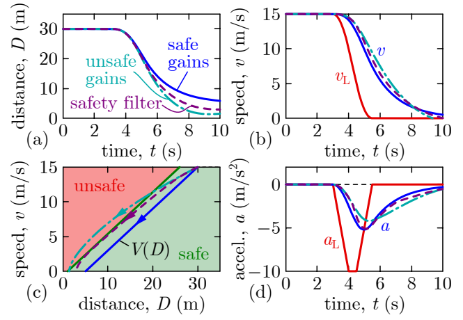
Fig. 2. Simulations of model (1) with CCC (2), using a provably safe choice of controller parameters (solid lines) and an unsafe choice (dash-dot lines). These sets of parameters correspond to points P and Q in Fig. 5(a), respectively. For the unsafe CCC setup, formal safety guarantees can be recovered by utilizing the safety filter (28)-(30) (dashed lines).
