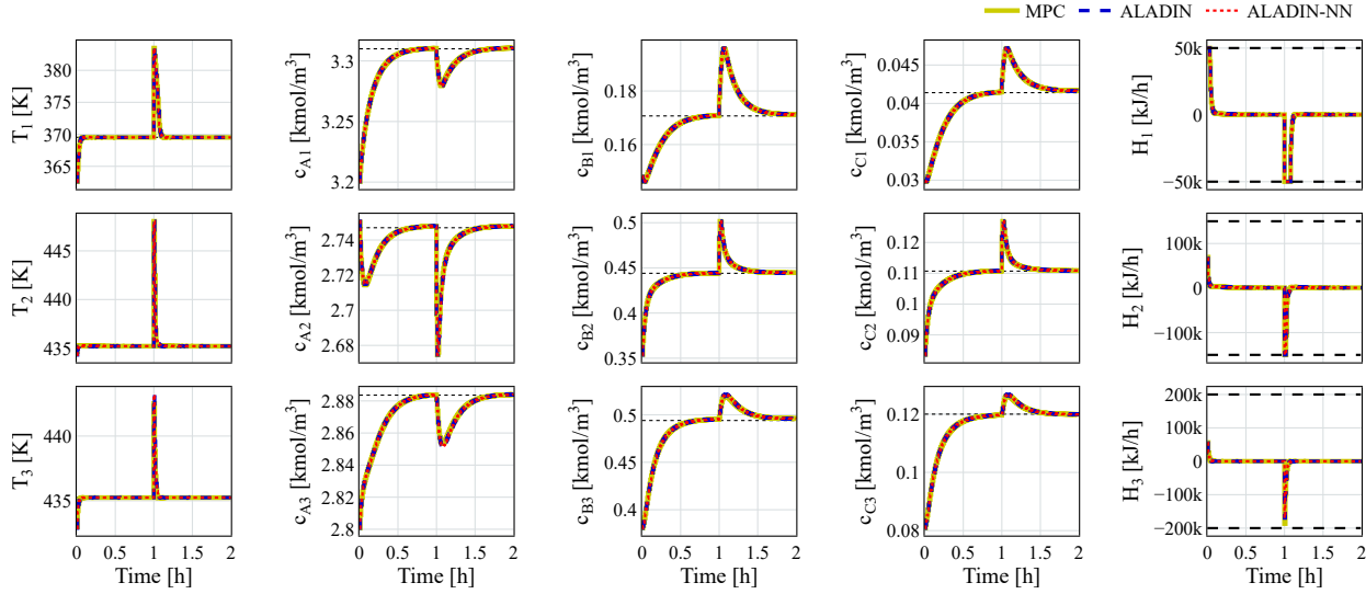
Fig. 2. From the left first four columns represents the system state control trajectories of closed-loop simulation: nominal MPC (yellow), rigorous ALADIN-based MPC (blue), proposed ALADIN-NN-based MPC (red), and steady-state reference x^s (black). The last column show closed-loop control profiles of the control inputs: nominal MPC (yellow), rigorous ALADIN-based MPC (blue), proposed ALADIN-NN-based MPC (red), and constraints (black).
