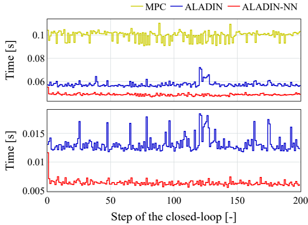
Fig. 3. Computational complexity of evaluated MPC design methods in closed-loop simulation: (i) upper plot: overall runtime, (ii) bottom plot: parallel elapsed time of the decoupled subproblems.
