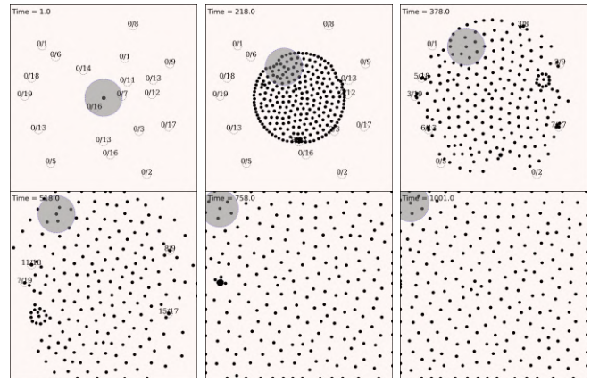
Fig. 1: Simulation of a target assignment scenario where targets disappear upon reaching the demanded number of agents. Agents move according to the electrostatic attraction-repulsion dynamics outlined in (17). The current time step is written in the top left corner of each frame. Agents' sensing range is depicted by the transparent gray disk (sensing range is depicted for a single agent to prevent visual clutter). 200 agents begin at the center of the region and expand outward, finding targets. The initial total demand of the targets is 204.
