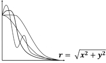
Fig. 2: Some possible choices of the signal function f(r) . Modifying f will alter the optimal agent signal coverage formation, hence also the agent dynamics.
